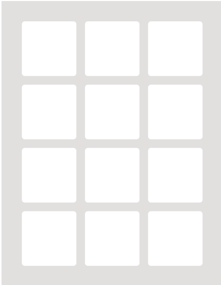
PRECAST PAVING PANEL 4 X 3 990 x 770 x 100
